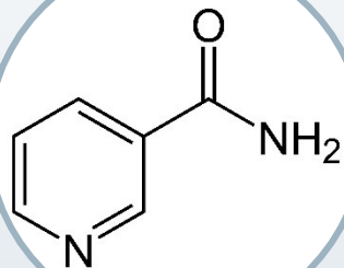
Nicotinamide
